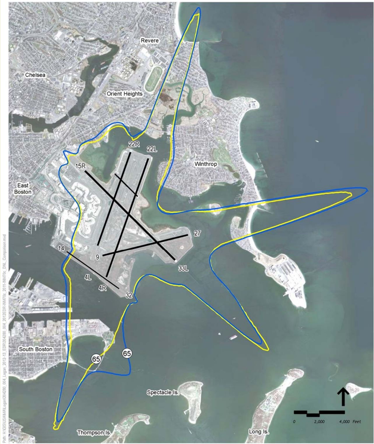
Figure 4: Comparison of the 65 dB DNL Contours for 2011 and 2012 Operations Using INM 7.0c
