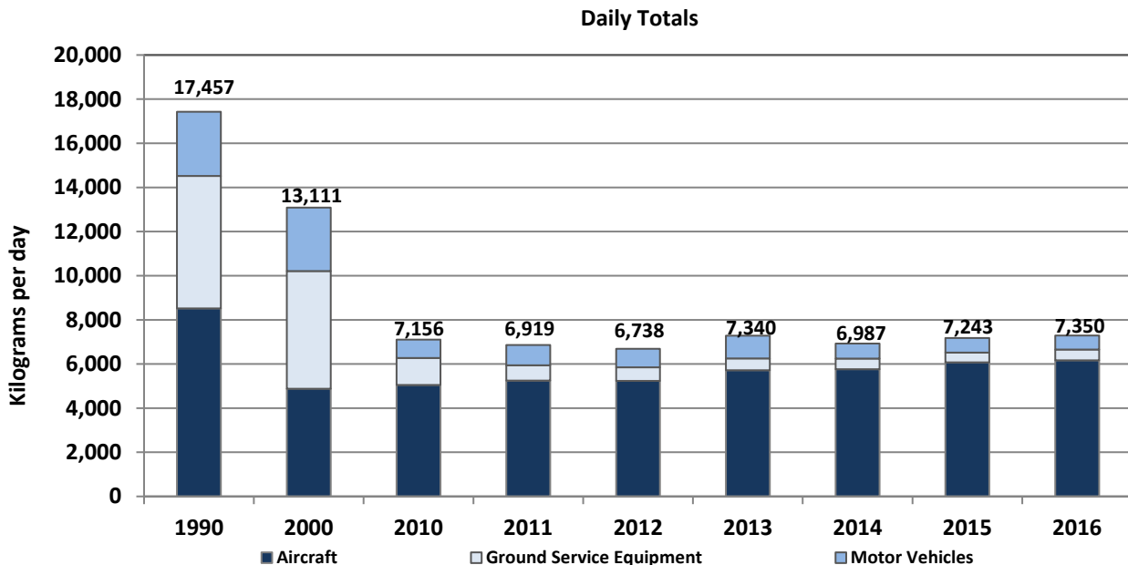
Figure 7-5 Modeled Emissions of CO at Logan Airport, 1990, 2000, and 2010-2016
