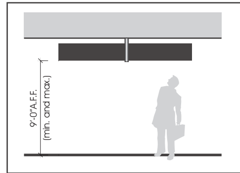
CEILING SUSPENDED
