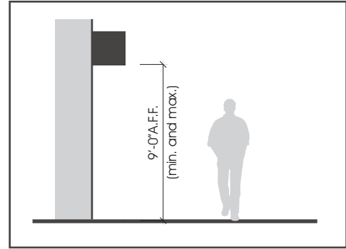
FLAG MOUNTED
