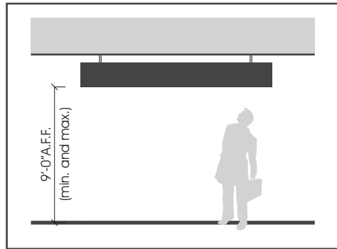
CEILING SUSPENDED
