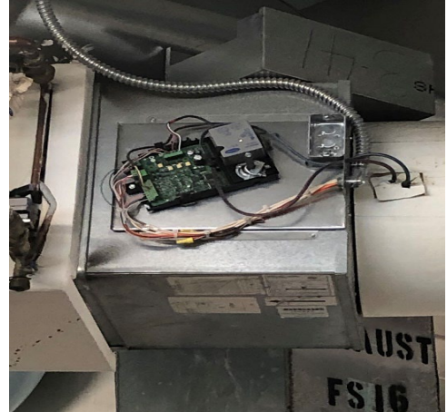
Fig. 15: DDC controls serve most of the HVAC terminal units within the bldgs. Constant Volume or Variable Air Volume units exist in the terminals.
